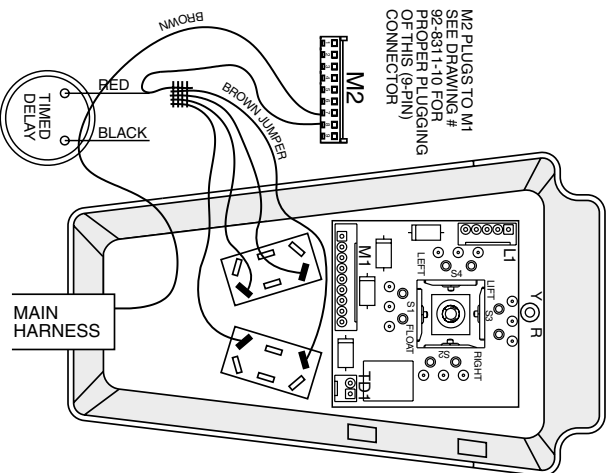
BROWN WIRE & BROWN JUMPER (92-8311-13)
