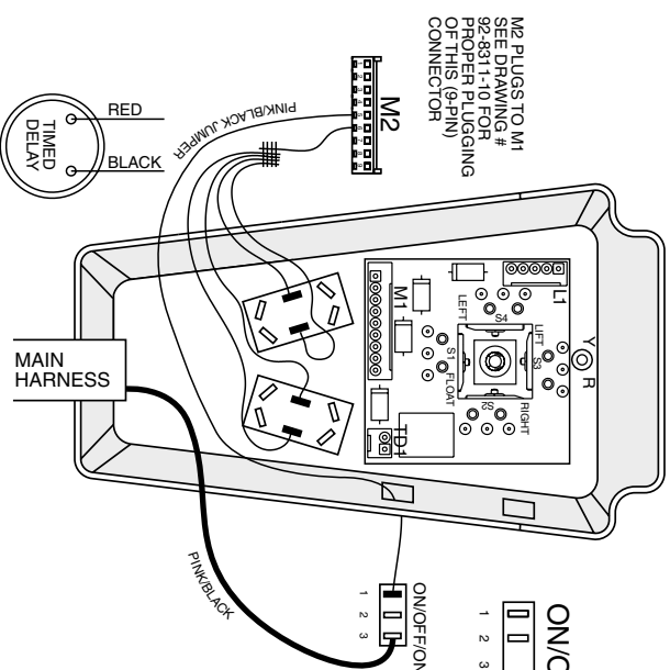
PINK/BLACK WIRE & PINK/BLACK JUMPERS 92-8311-11 & 92-8311-12
