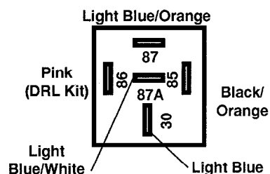
Driver-Side Headlamp Relay
