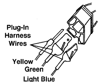
Driver-Side Vehicle Headlamp Connector
