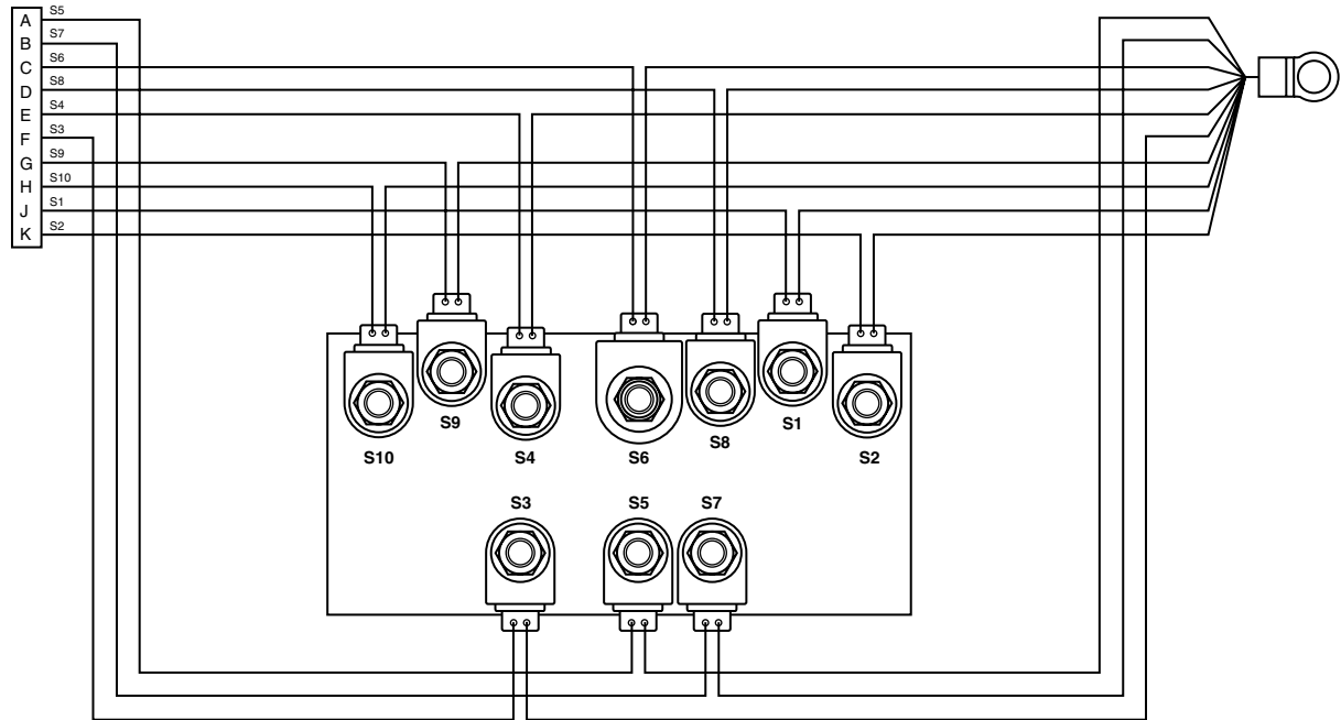
MODEL 810 COIL HARNESS (P/N 62120) WIRE SCHEMATIC (2001-2002)
