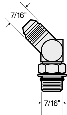
7/16"-20 x 7/16"-20 45° Adjustable Elbow O.R.B. Adapter
