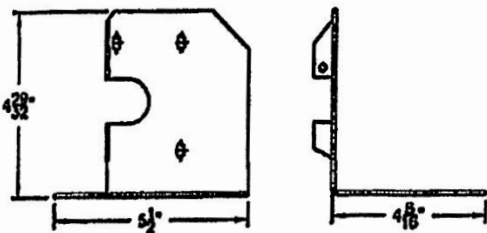
(7) E66HT HONDA THROTTLE BRACKET
